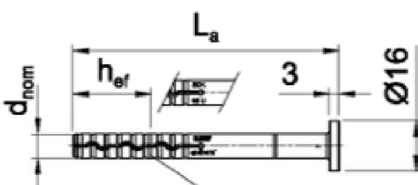
marking of effective anchoring depth
